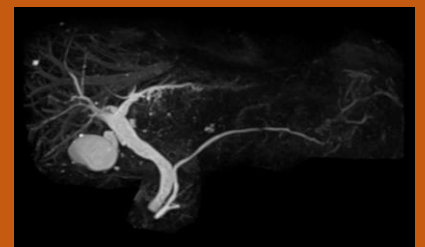
MRCP
